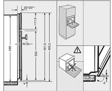
DGC 6600, DGC 6800, DGC 6805 detailed installations drawing for PureLine (Installation drawing)
